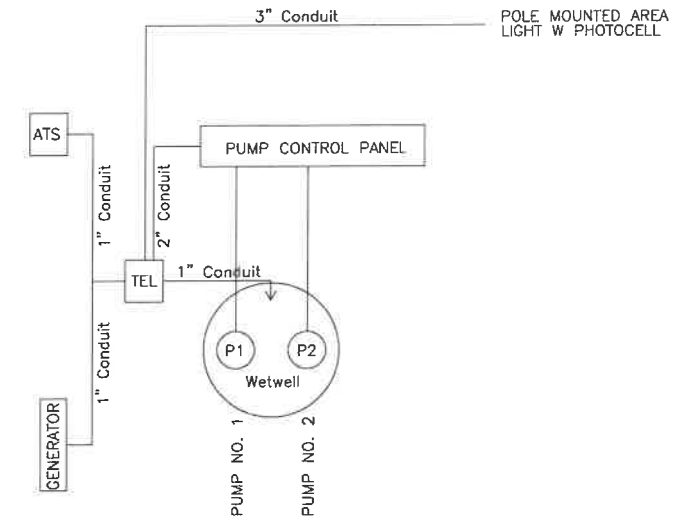
TYPICAL SCADA ONE-LINE DIAGRAM DETAIL S 11a NO SCALE
