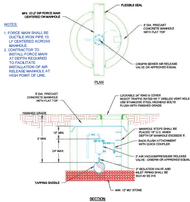
TYPICAL AIR VACUUM/RELEASE MANHOLE FOR FORCE MAIN DETAIL S 19 NO SCALE
