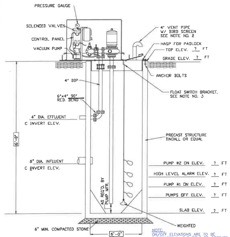
TYPICAL SEWER LIFT STATION PROFILE FOR ABOVE GROUND PUMPS DETAIL S 4 NO SCALE
