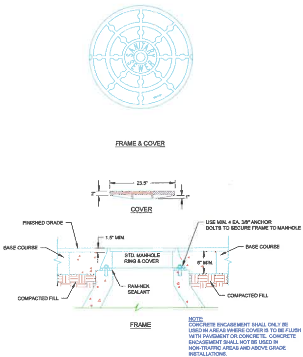
TYPICAL STANDARD MANHOLE FRAME & COVER DETAIL S 21 NO SCALE
