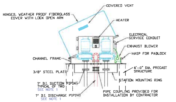
TYPICAL PUMP ELEVATION FOR SEWER LIFT STATION WITH ABOVE GROUND PUMPS DETAIL S 5 NO SCALE
