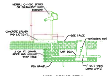
TYPICAL YARD HYDRANT INSTALLATION DETAIL S 6 NO SCALE
