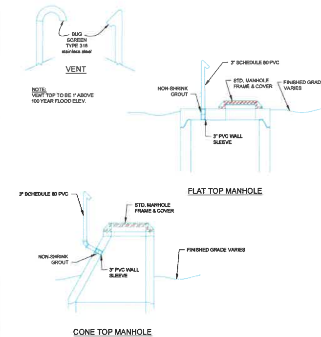
TYPICAL VENTED MANHOLE DETAIL S 23 NO SCALE
