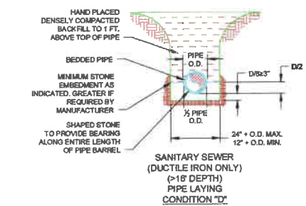
TYPICAL PIPE LAYING CONDITION DETAIL S 17 NO SCALE
