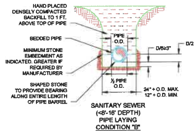
TYPICAL PIPE LAYING CONDITION DETAIL S 16 NO SCALE
