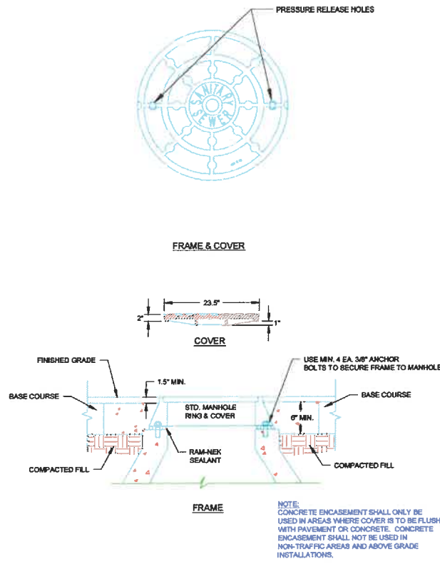
TYPICAL PRESSURE RELEASE MANHOLE FRAME & COVER DETAIL S 20 NO SCALE
